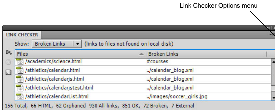
Figure 1 Link Checker tab
